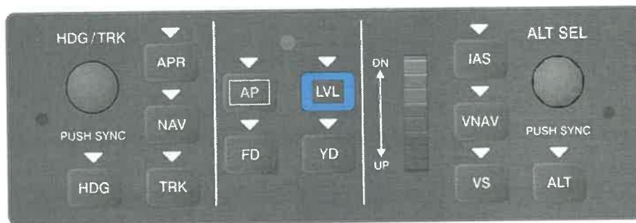
Figure 7-3: GMC 507 Control Unit (Reference Only)
