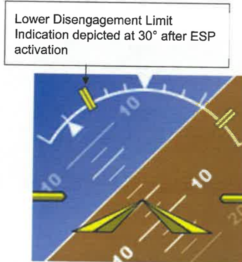
Figure 7-2: Engagement Limit Indications Upon ESP Activation
